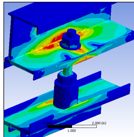
FEA analysis showing the CPR under load
