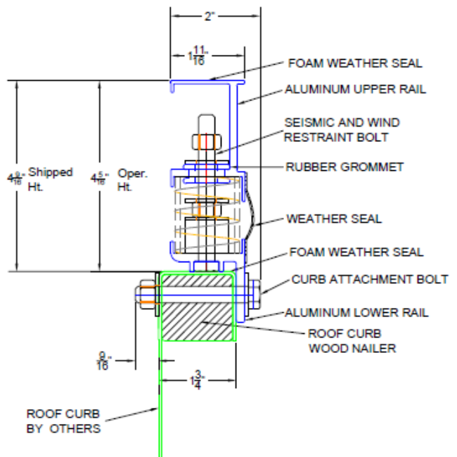
CPR-1 Cross Section View
